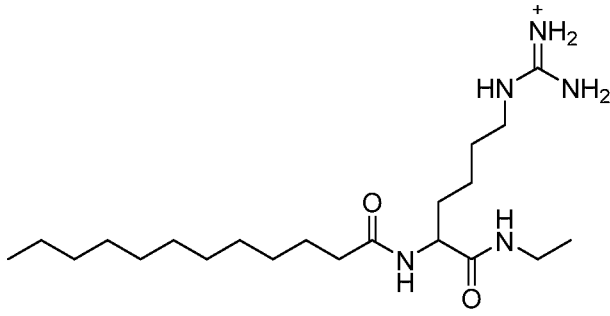
[amino({[5-dodecanamido-5-(ethylcarbamoyl)pentyl]amino})methylidene]azanium
