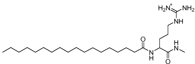
[amino({[4-(methylcarbamoyl)-4-octadecanamidobutyl]amino})methylidene]azanium
