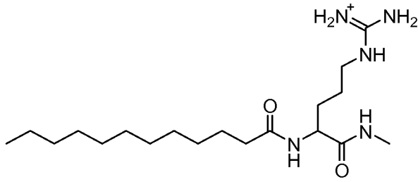
[amino({[4-dodecanamido-4-(methylcarbamoyl)butyl]amino})methylidene]azanium
