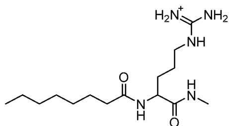
[amino({[4-(methylcarbamoyl)-4-octanamidobutyl]amino})methylidene]azanium
