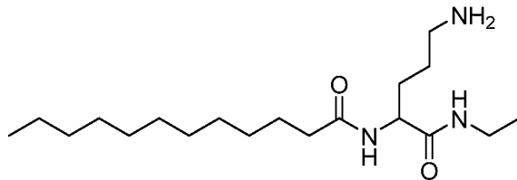
N-[4-amino-1-(ethylcarbamoyl)butyl]dodecanamide
