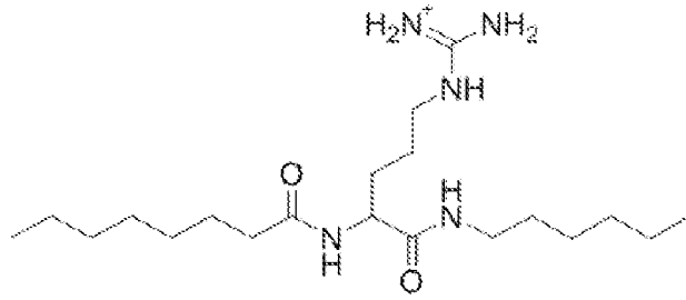
[amino({[4-(hexylcarbamoyl)-4-octanamidobutyl]amino})methylidene]azanium
