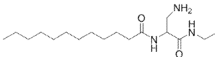
N-[2-amino-1-(ethylcarbamoyl)ethyl]dodecanamide
