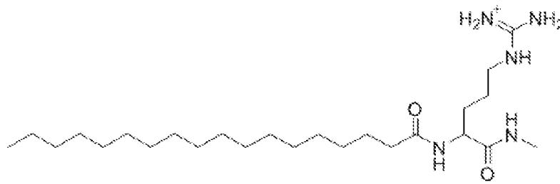
[amino([4-(methylcarbamoyl)-4-octadecanamidobutyl]amino)methylidene]azanium
