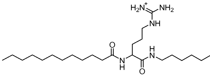
[amino({[4-dodecanamido-4-(hexylcarbamoyl)butyl]amino})methylidene]azanium
