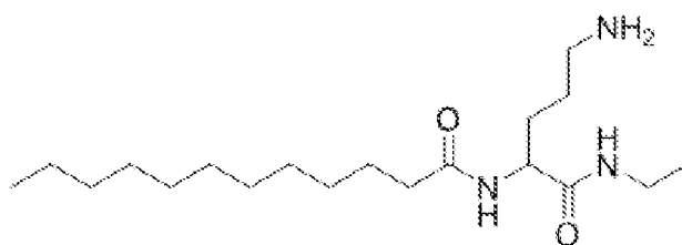
N-[4-amino-1-(ethylcarbamoyl)butyl]dodecanamide
