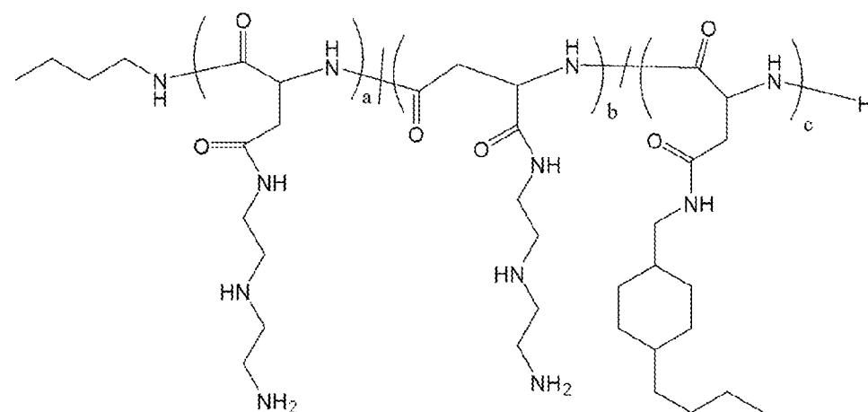
Polymer 9
