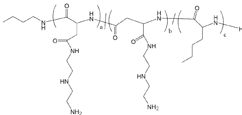
Polymer 5
