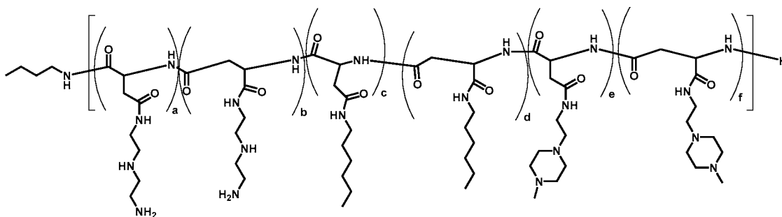
Polymer 49
