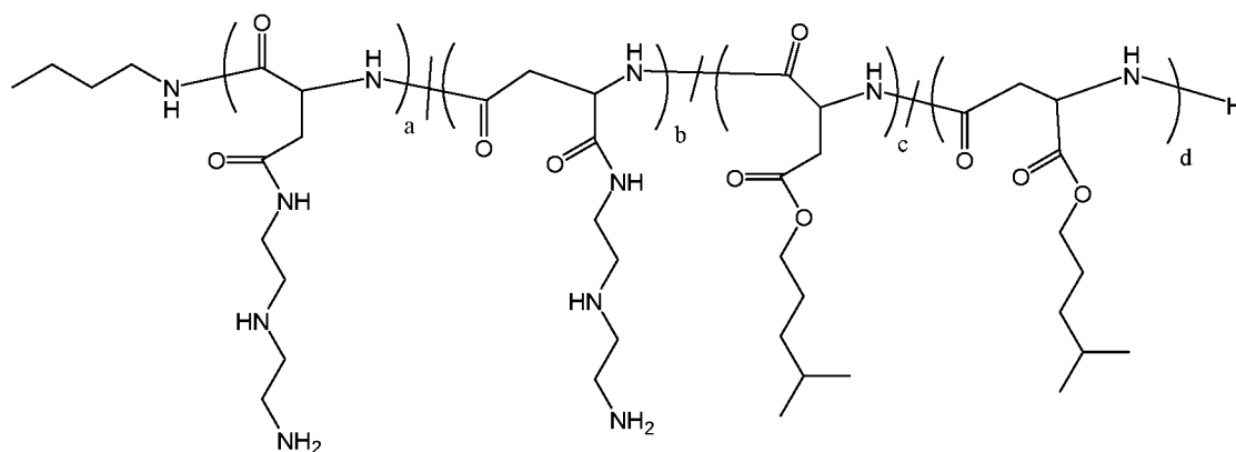
Polymer 34
