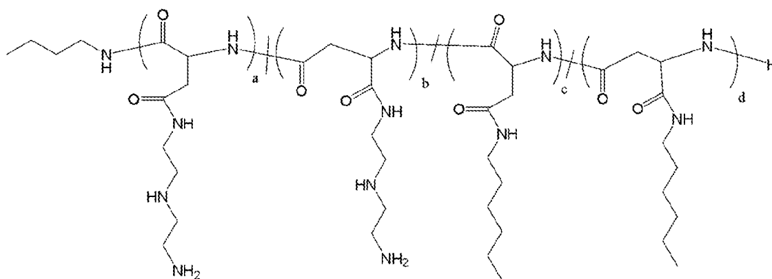
Polymer 13
