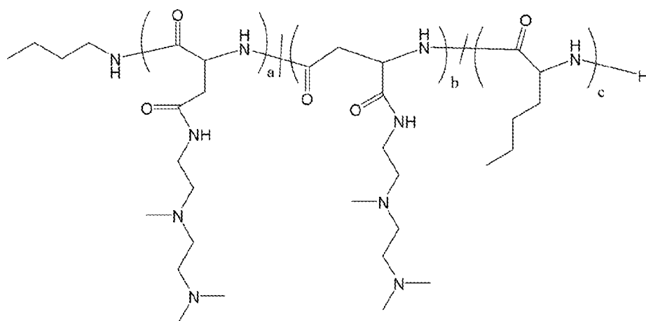
Polymer 21
