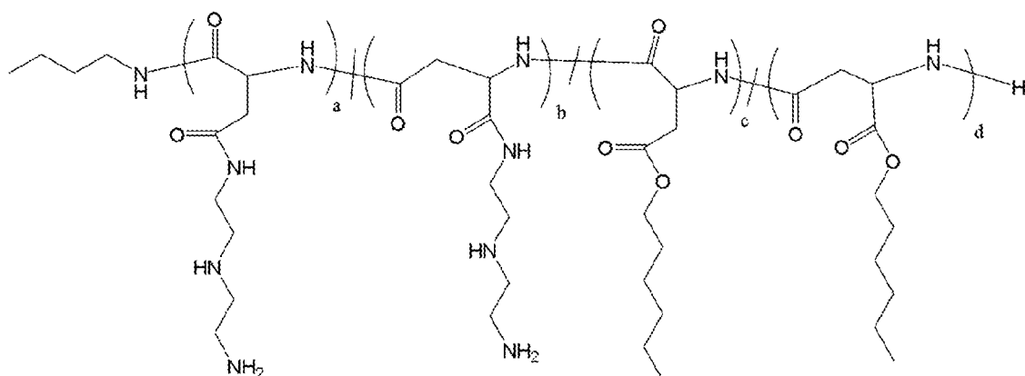
Polymer 14
