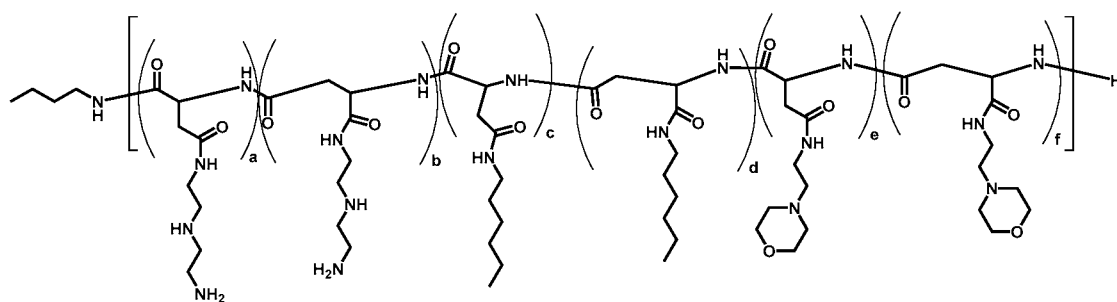
Polymer 48
