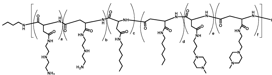
Polymer 57
