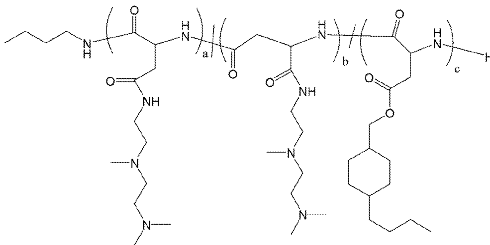
Polymer 26
