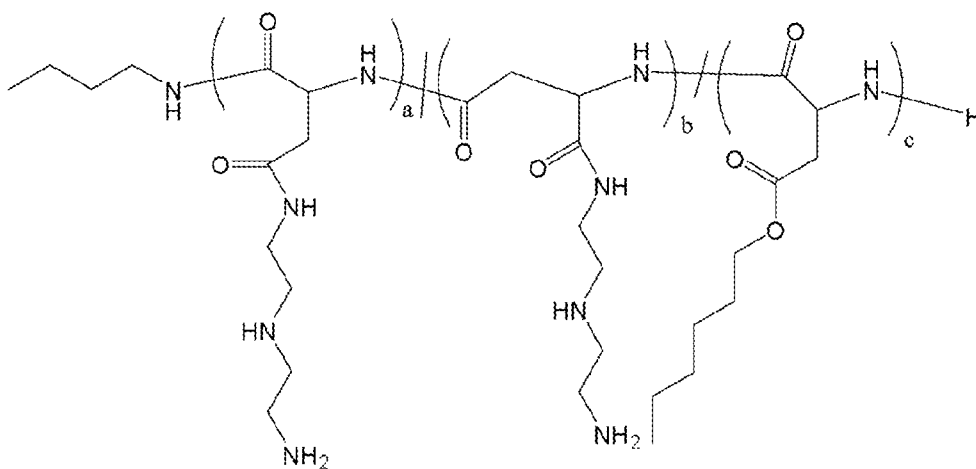
Polymer 4
