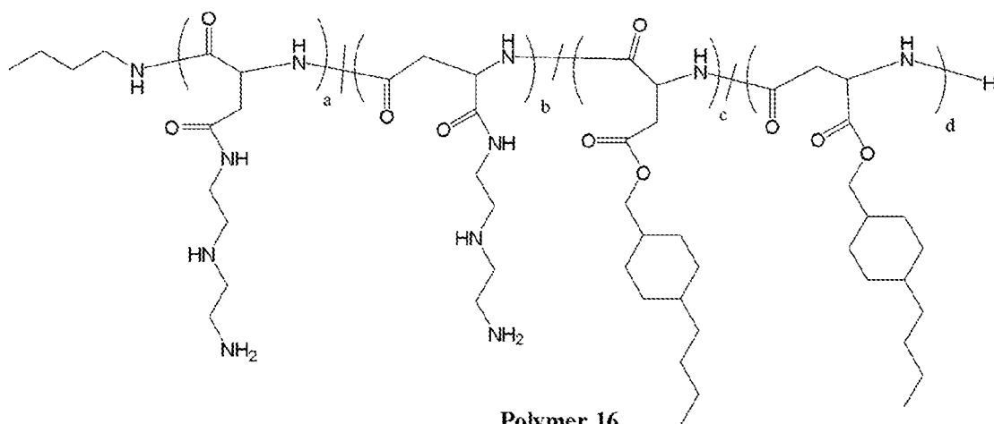
Polymer 16
