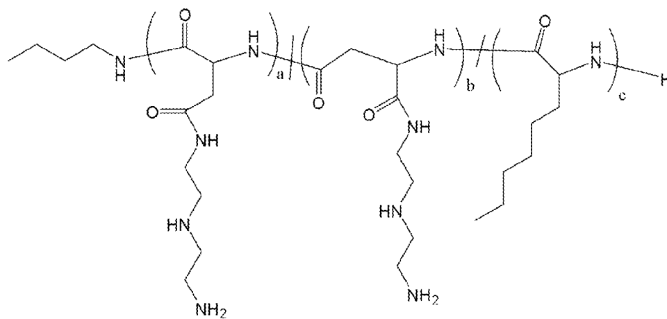
Polymer 1
