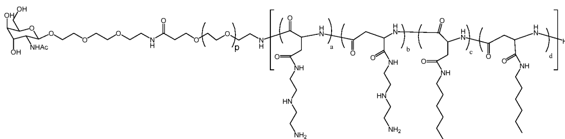
Polymer 69
