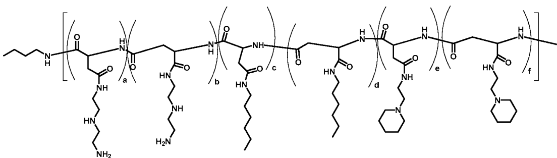
Polymer 47
