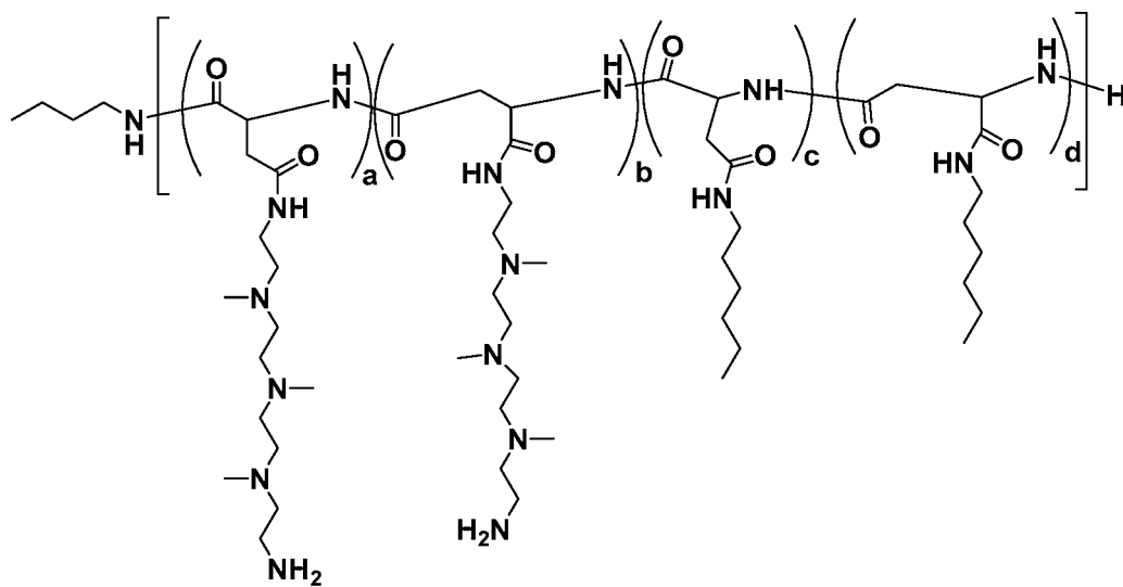
Polymer 42
