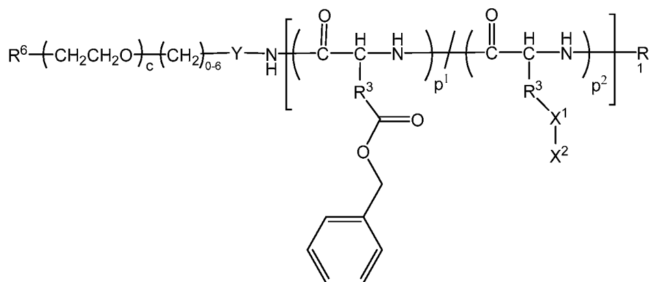
Formula 3A
