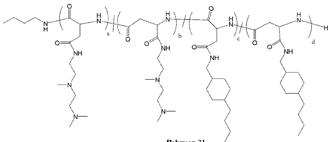
Polymer 31
