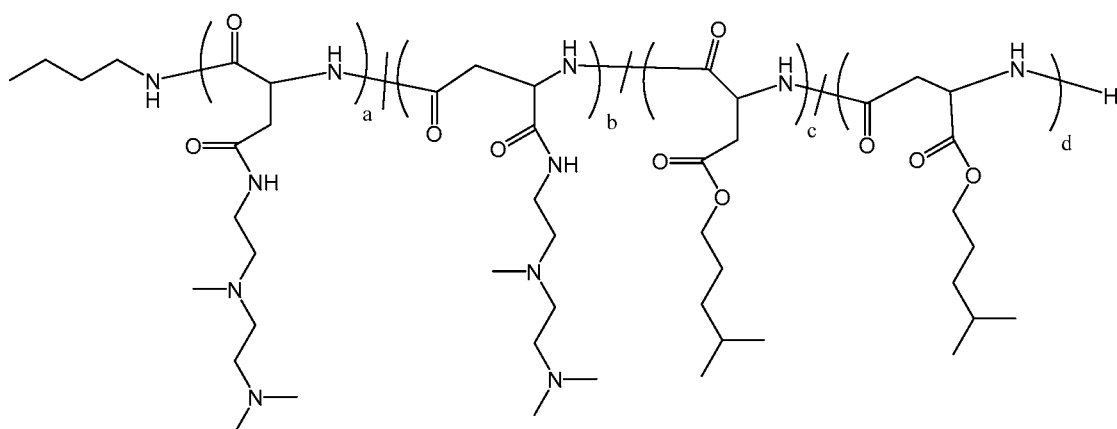
Polymer 36
