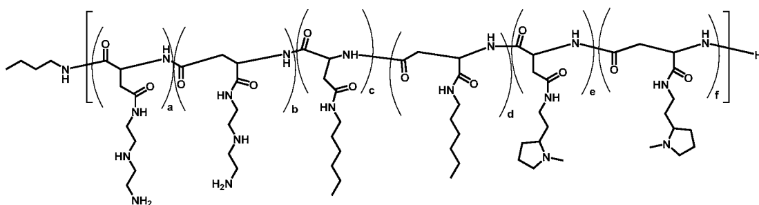
Polymer 50
