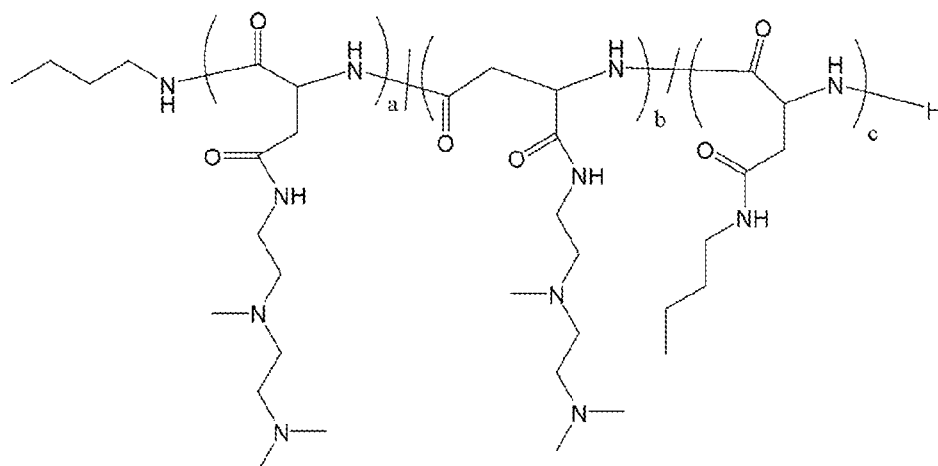
Polymer 23
