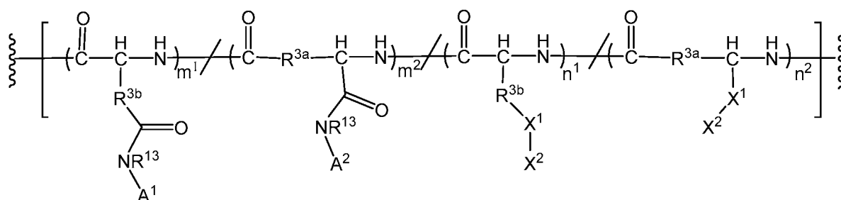
Formula 4
