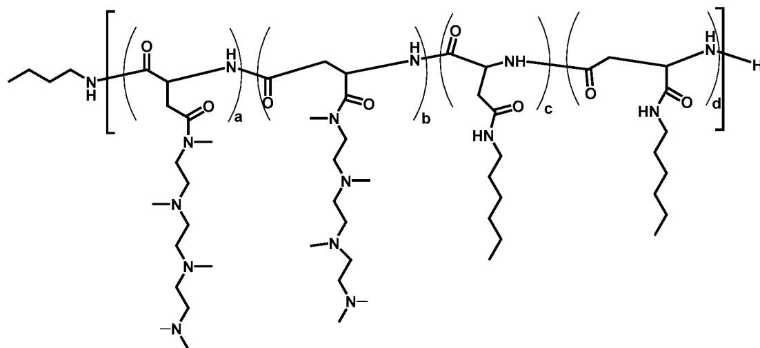
Polymer 38
