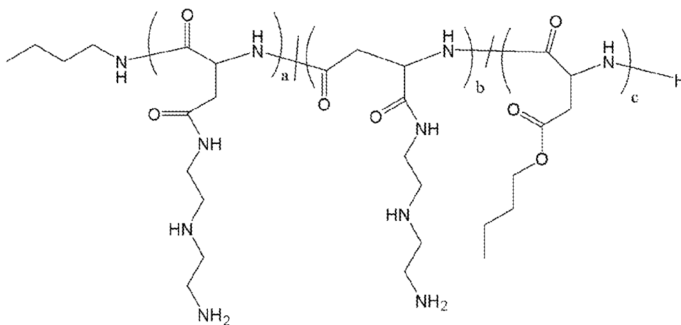
Polymer 8
