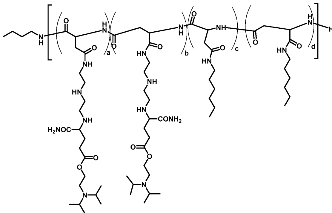
Polymer 67
