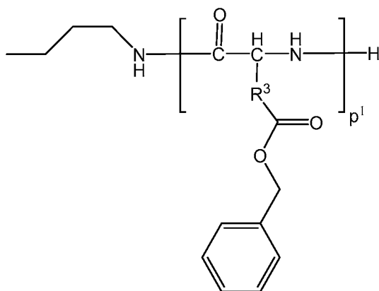
Formula 2B
