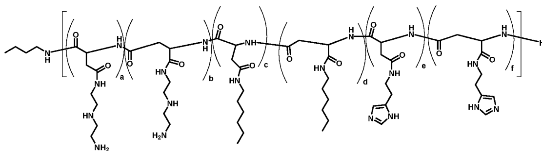
Polymer 51
