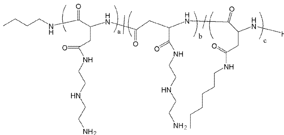
Polymer 3
