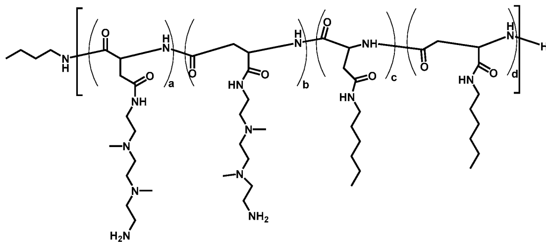
Polymer 41
