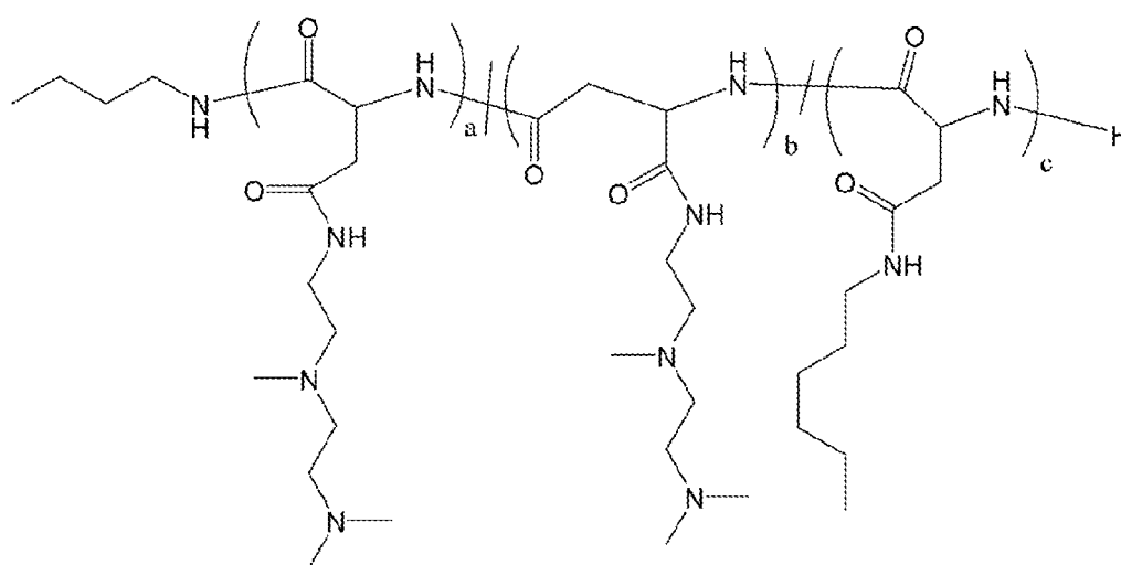
Polymer 19
