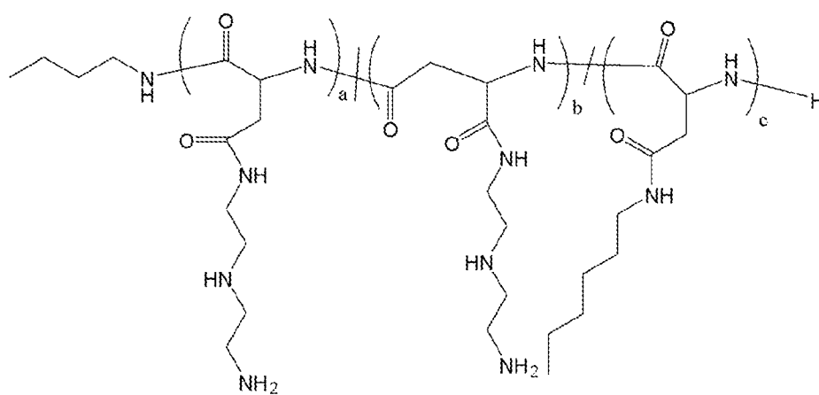
Polymer 3
