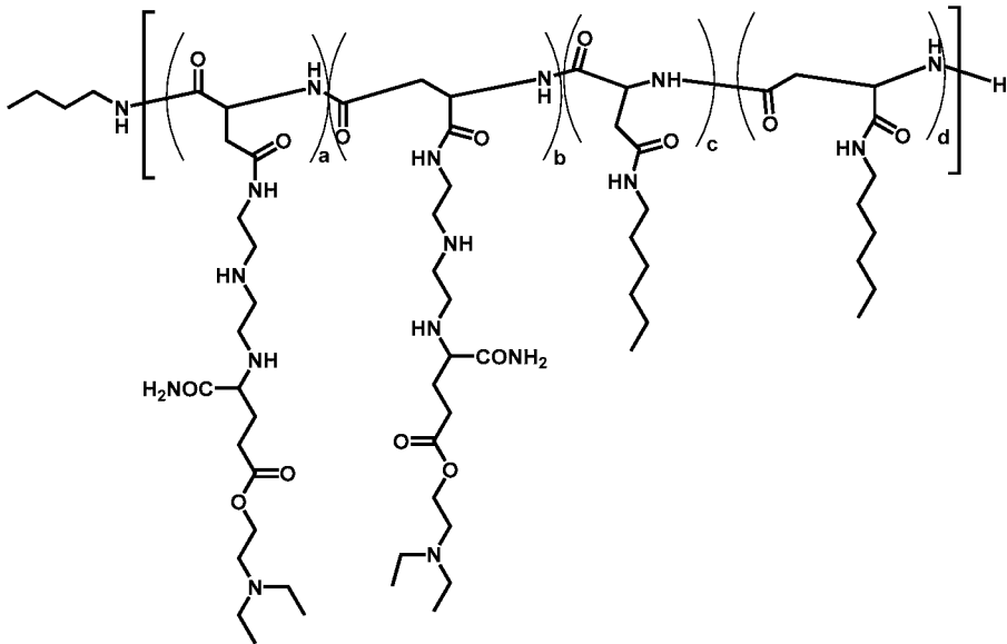
Polymer 63
