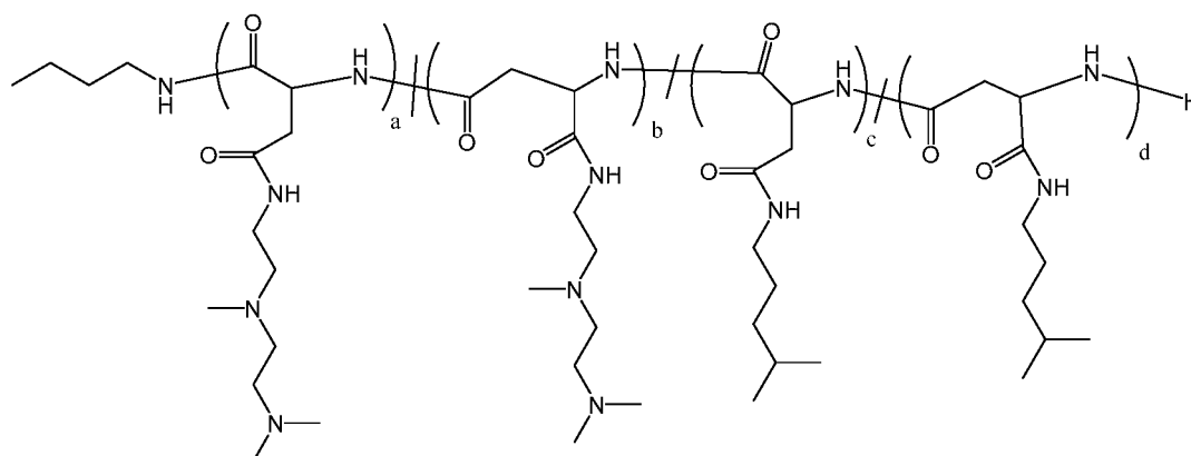
Polymer 35
