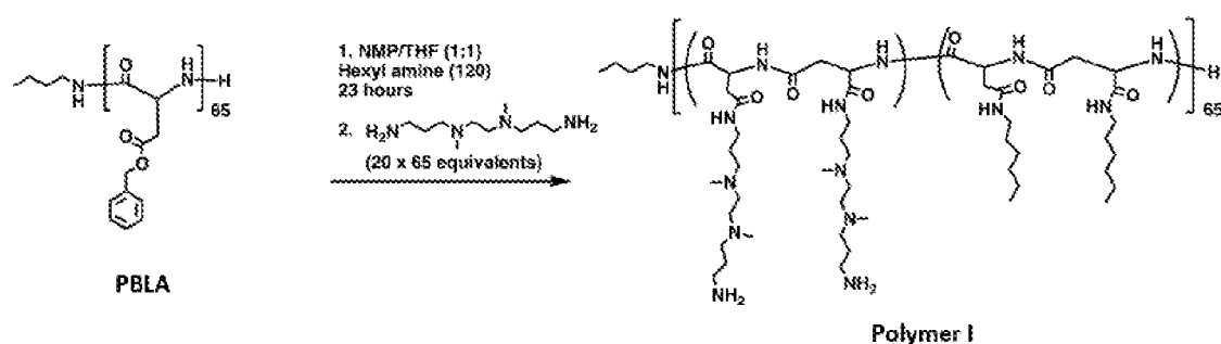
Scheme 15: Synthesis of Polymer I
