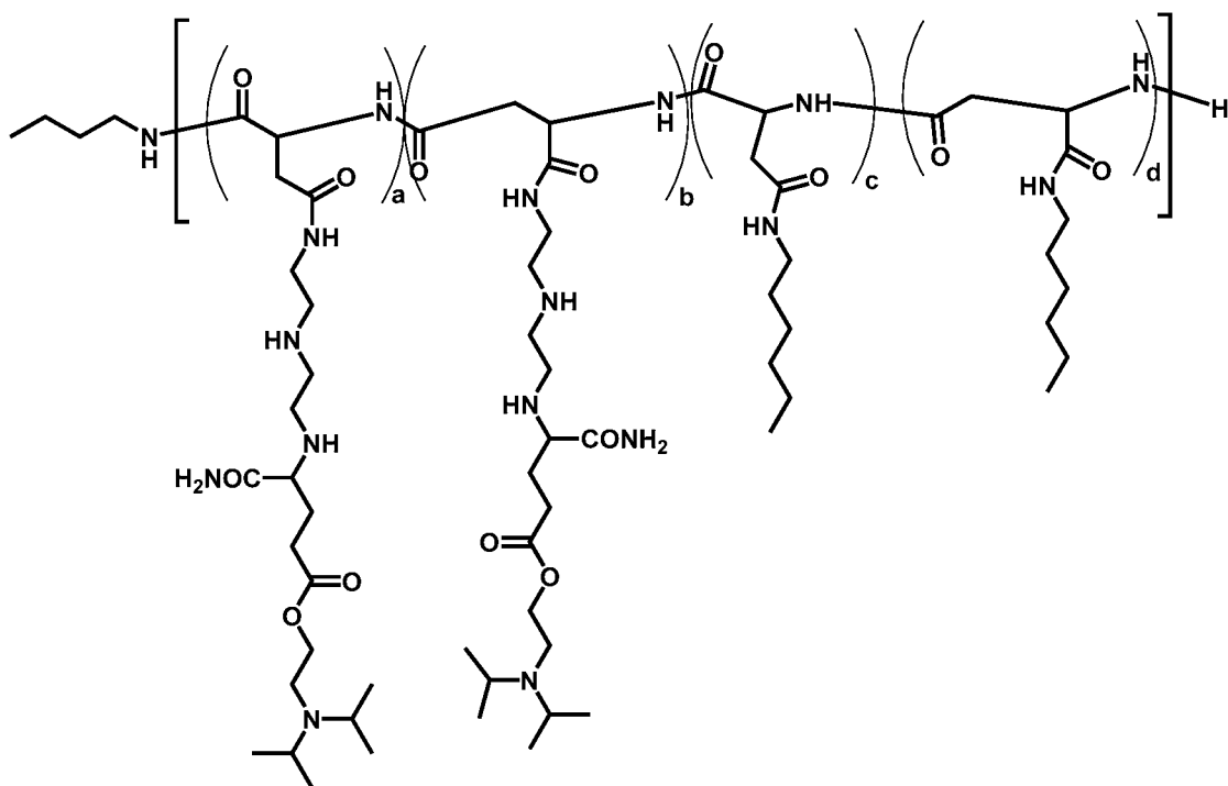
Polymer 67
