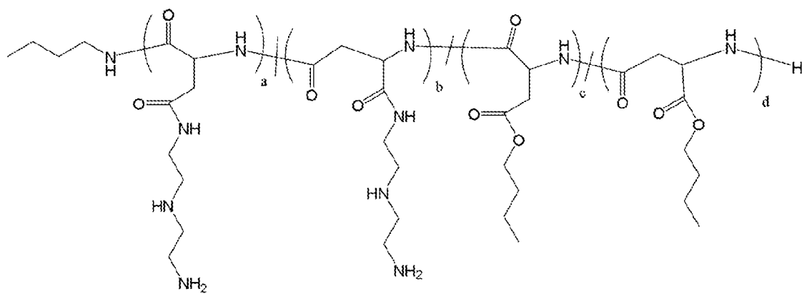
Polymer 12
