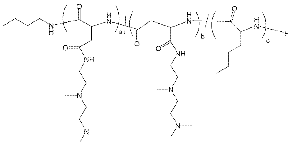
Polymer 21
