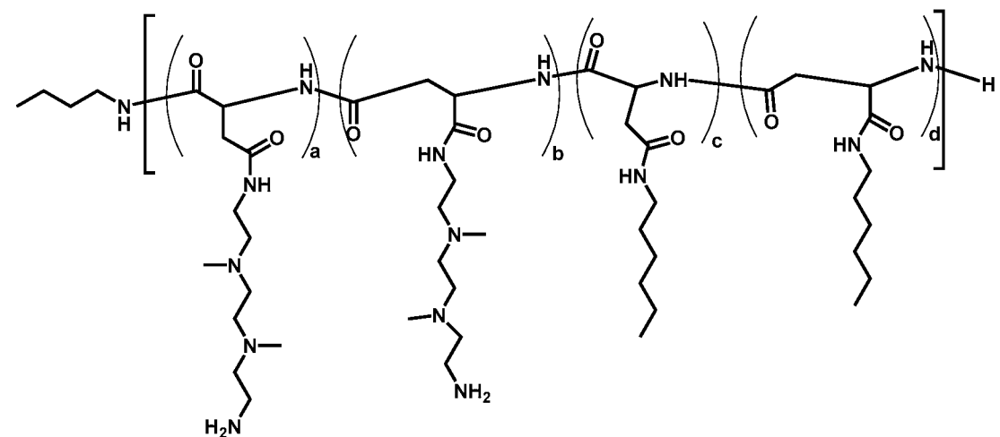
Polymer 41
