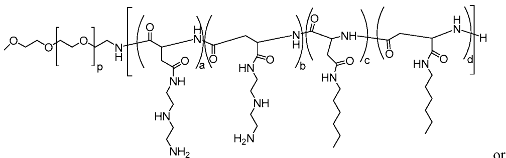
Polymer 68
