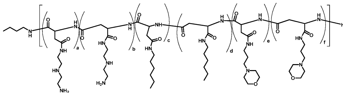
Polymer 56
