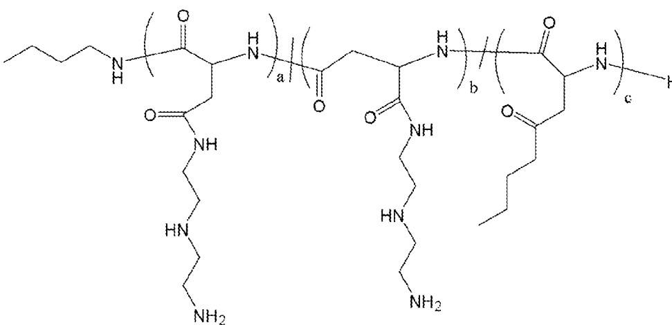
Polymer 6
