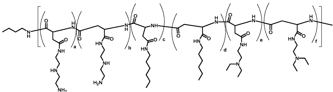
Polymer 45
