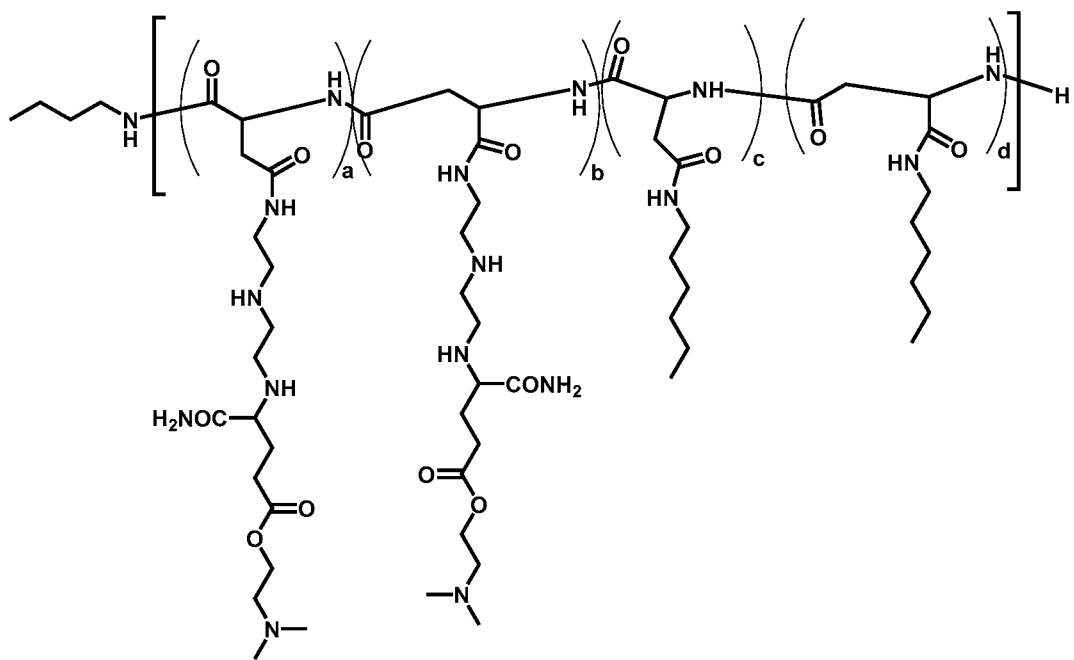
Polymer 66
