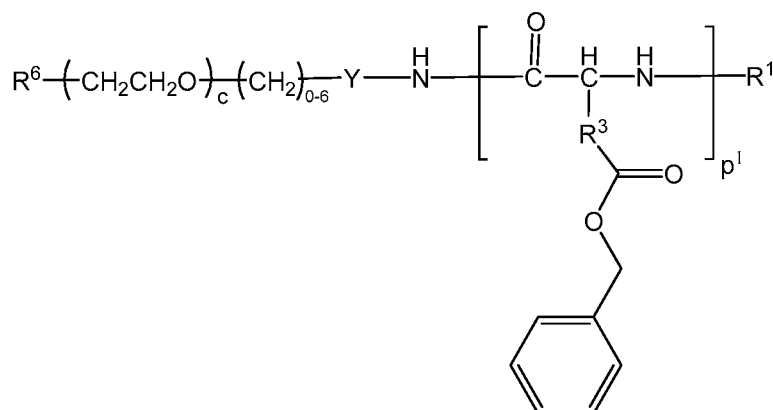
Formula 2A
