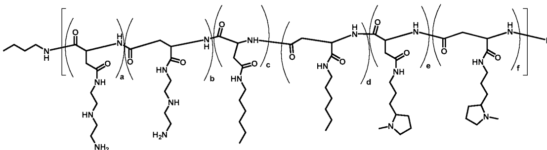
Polymer 58
