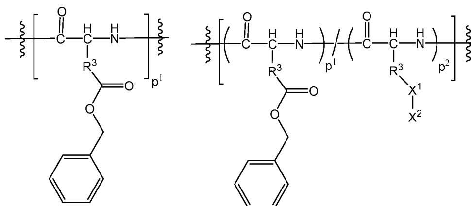
Formula 2
