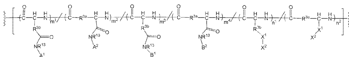
Formula 4
