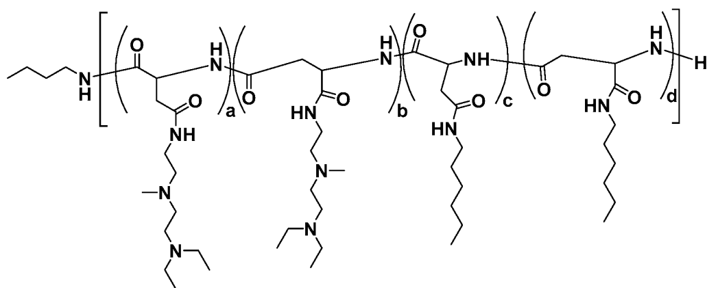
Polymer 43
