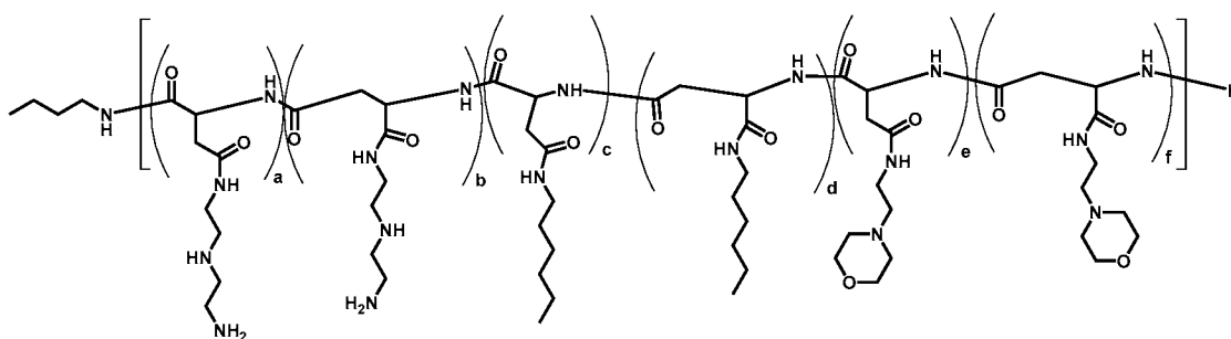
Polymer 48
