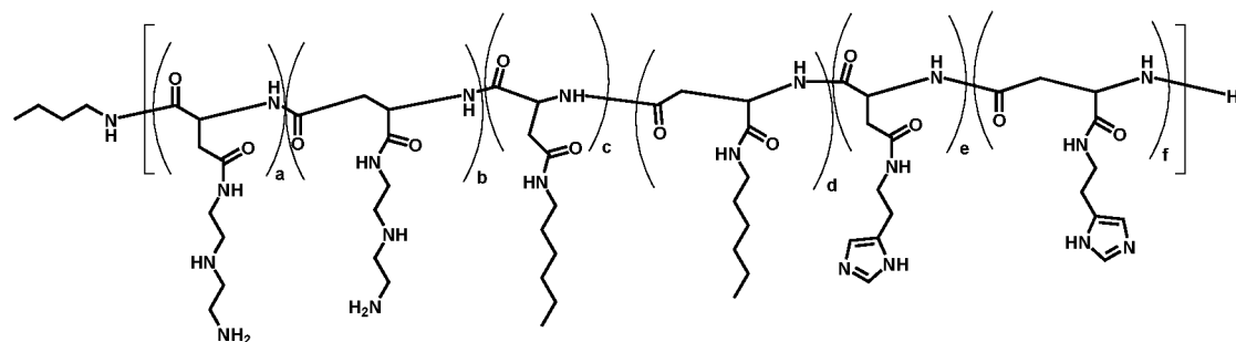
Polymer 51
