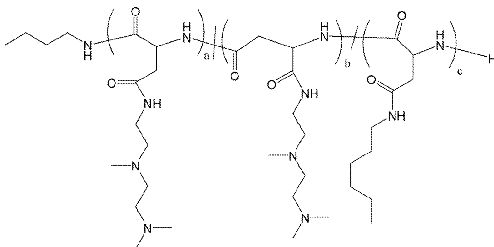
Polymer 19
