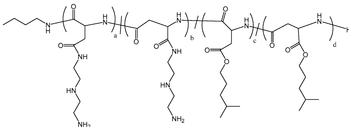
Polymer 34
