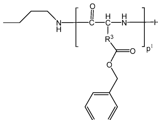
Formula 2B
