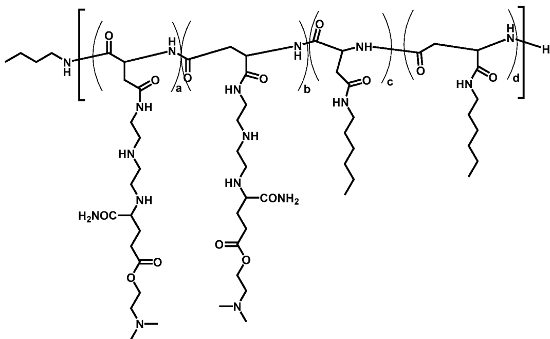
Polymer 66
