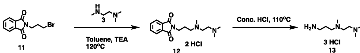
Scheme 7: Synthesis of Amine Compound 13
