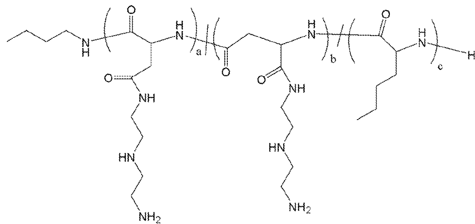
Polymer 5
