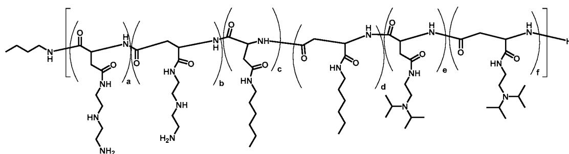
Polymer 46
