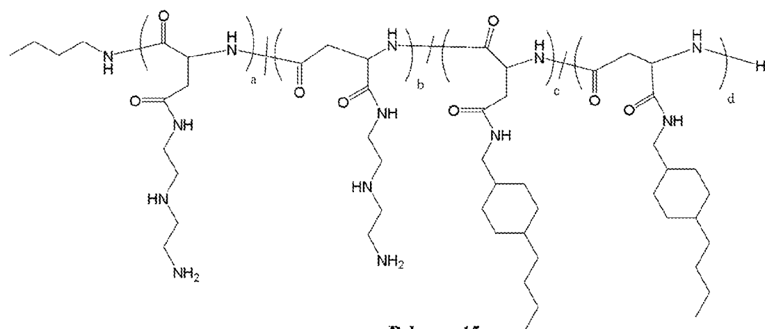
Polymer 15
