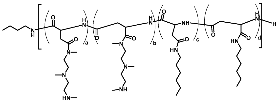
Polymer 40
