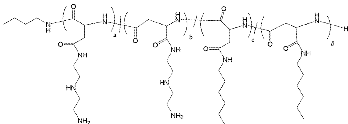
Polymer 13
