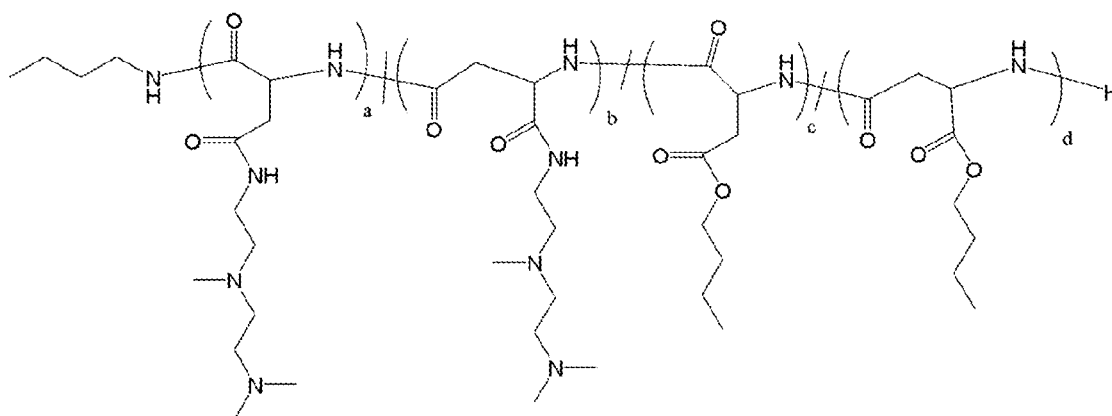
Polymer 28
