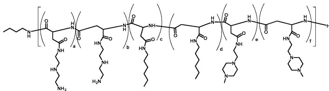
Polymer 49
