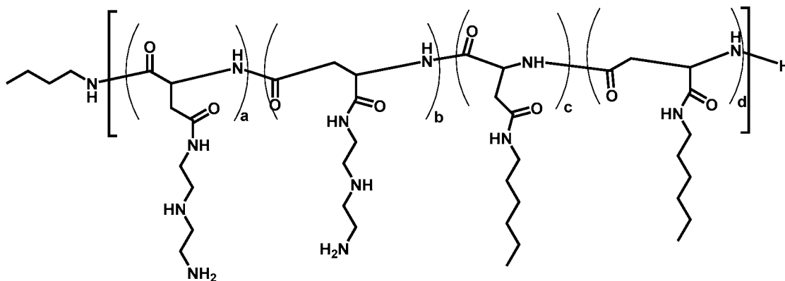
Polymer 37
