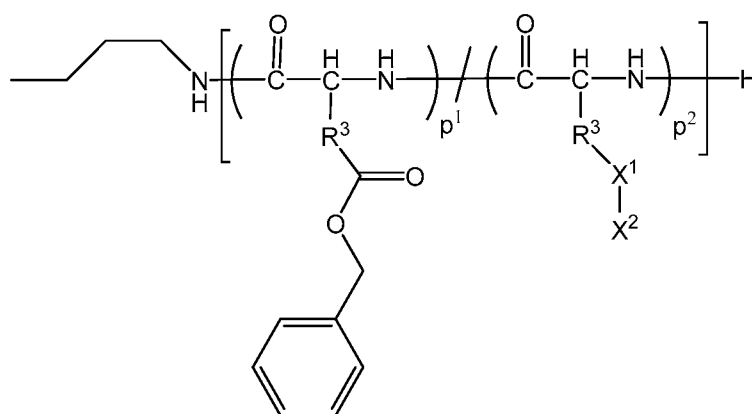
Formula 3B
