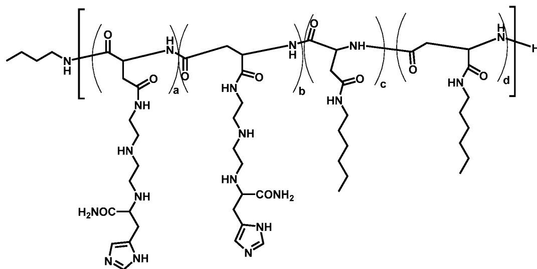
Polymer 60
