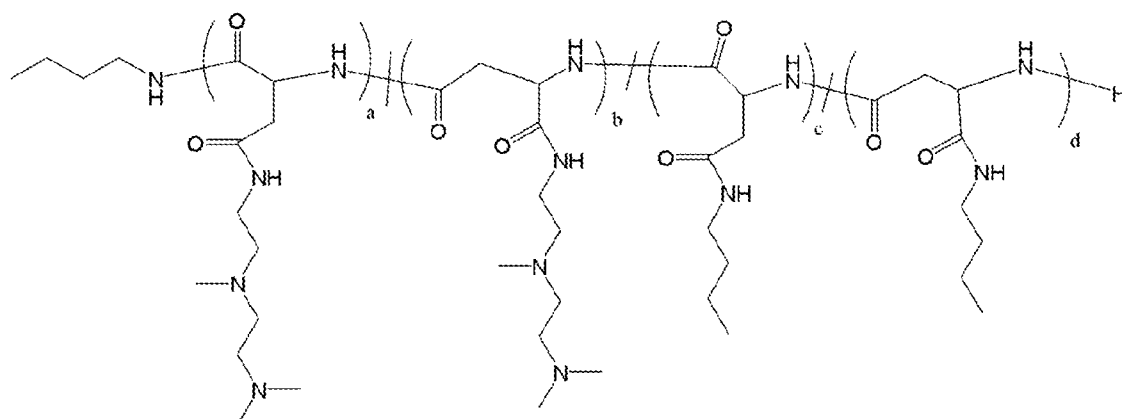
Polymer 27
