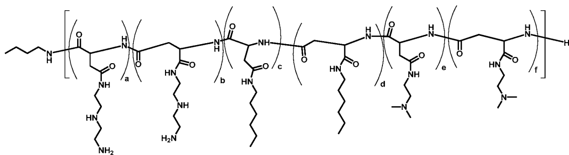
Polymer 44
