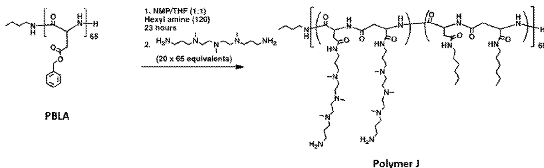
Scheme 17: Synthesis of Polymer J
