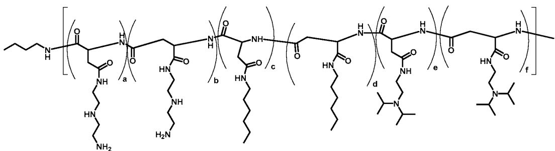
Polymer 46
