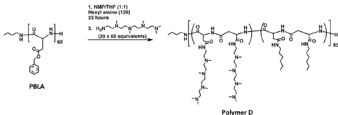
Scheme 6: Synthesis of Polymer D:
