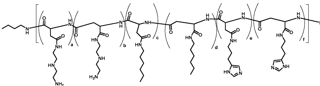
Polymer 59
