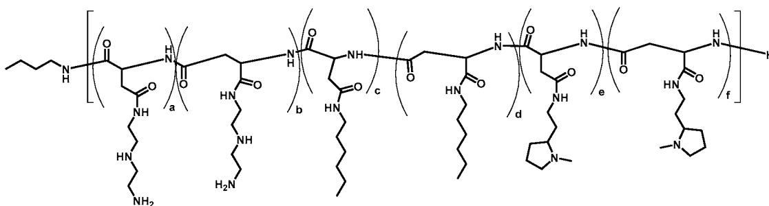
Polymer 50
