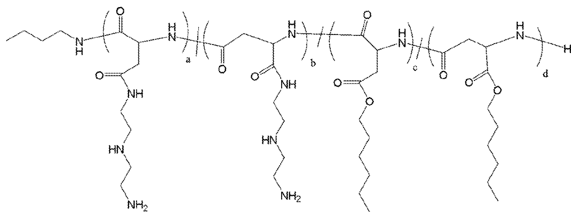
Polymer 14
