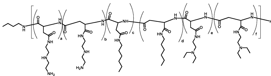
Polymer 45
