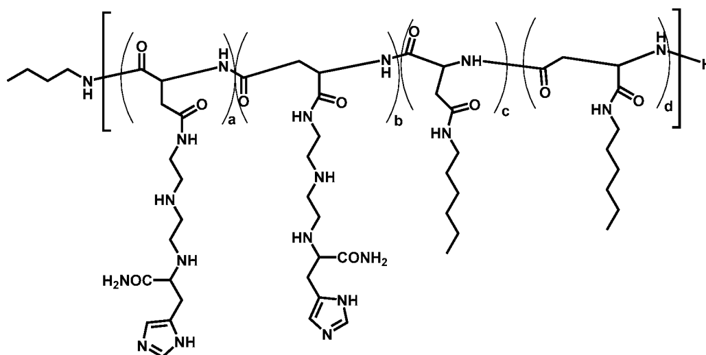
Polymer 60
