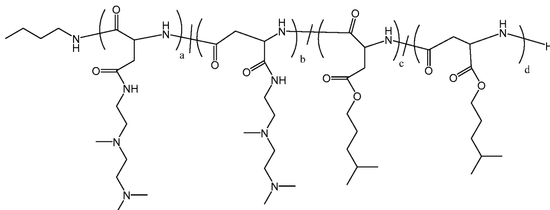
Polymer 36
