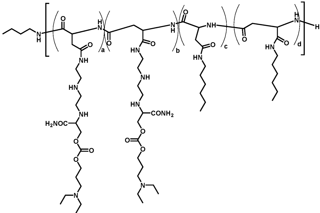
Polymer 62
