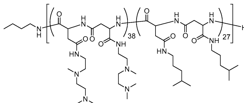
Polymer C
