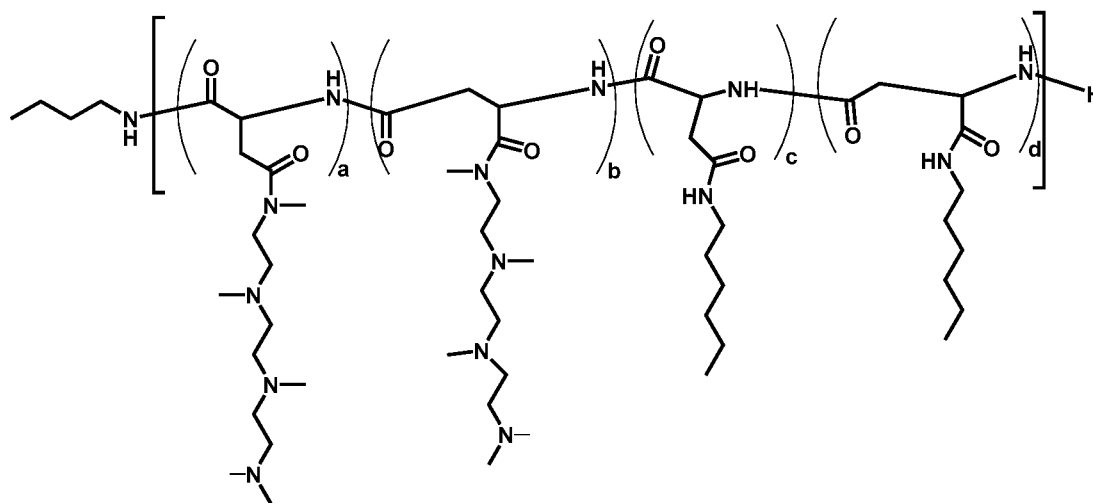
Polymer 38
