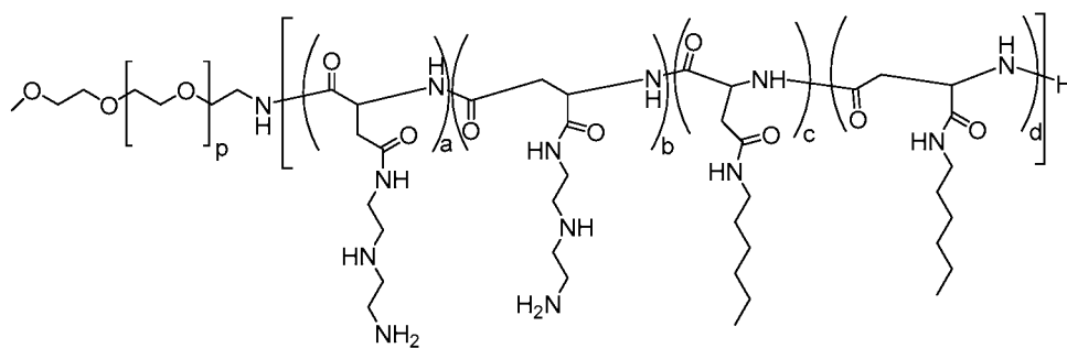
Polymer 68
