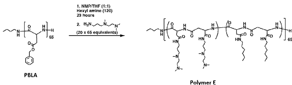
Scheme 8: Synthesis of Polymer E
