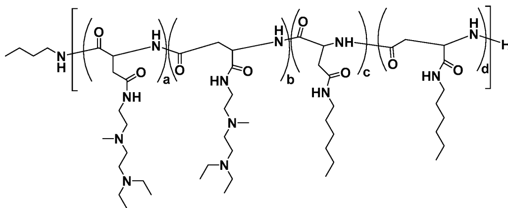
Polymer 43
