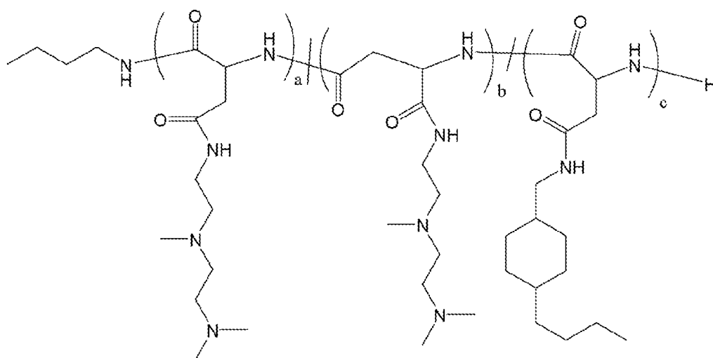
Polymer 25
