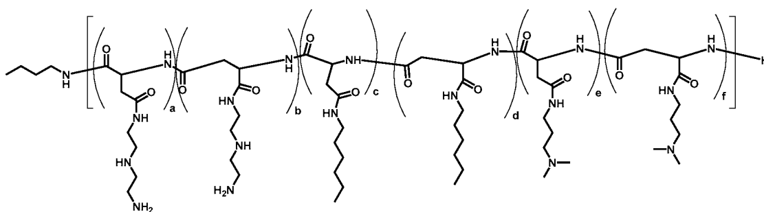
Polymer 52
