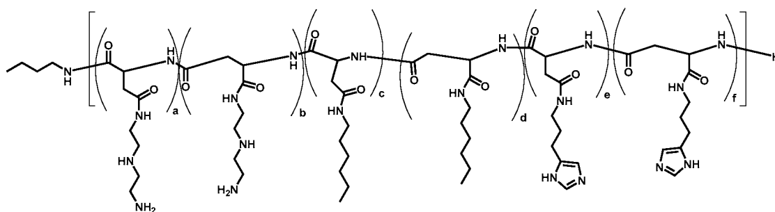
Polymer 59
