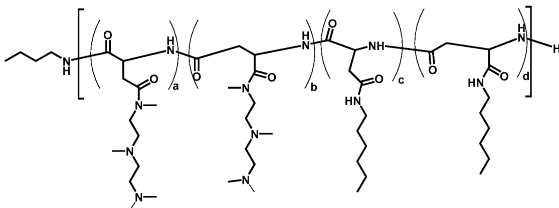
Polymer 39
