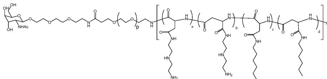
Polymer 69
