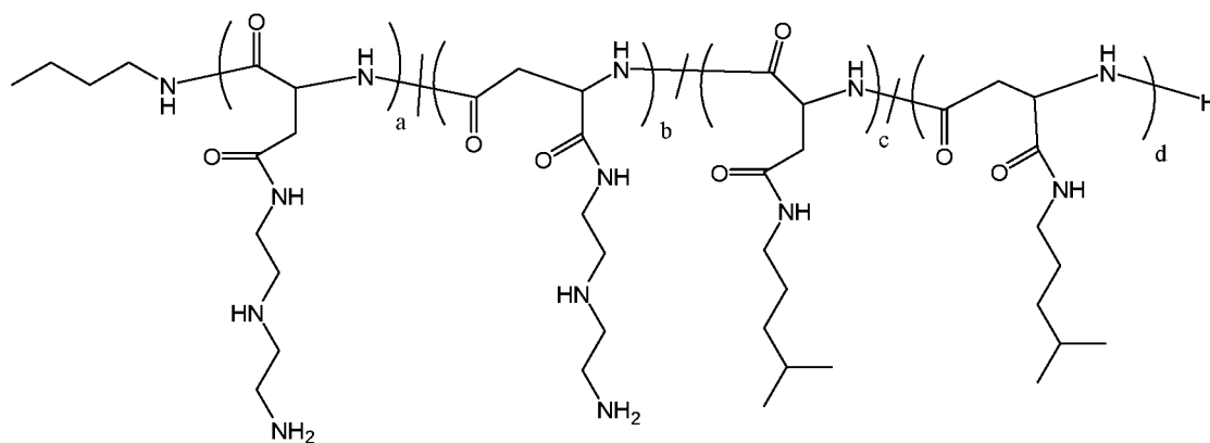
Polymer 33
