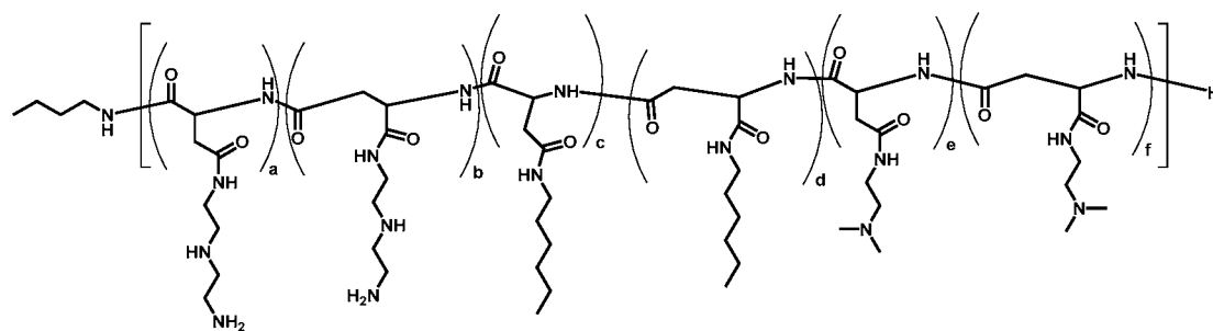
Polymer 44
