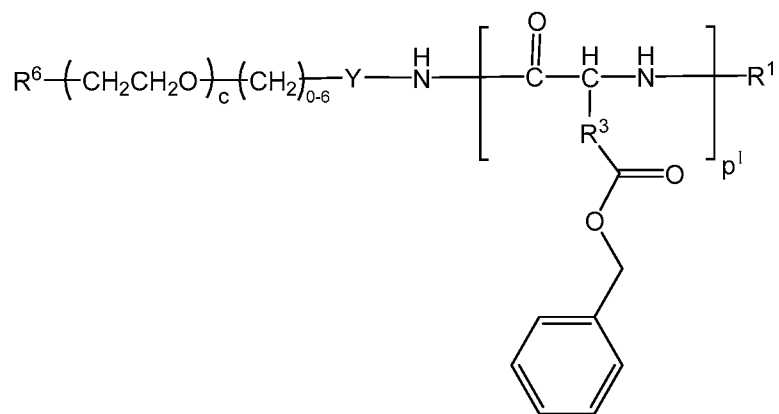
Formula 2A
