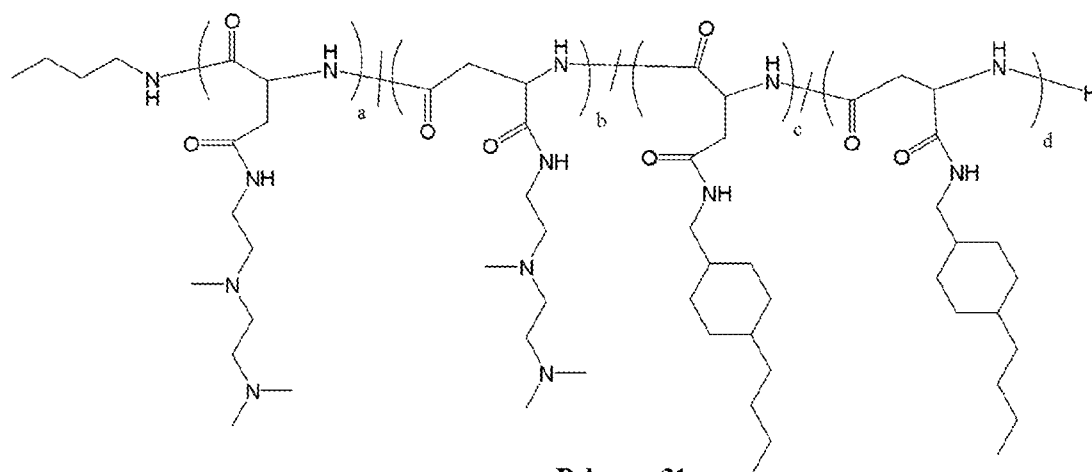
Polymer 31
