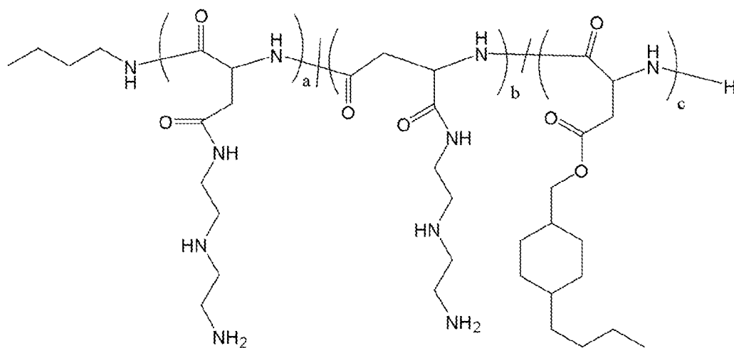
Polymer 10
