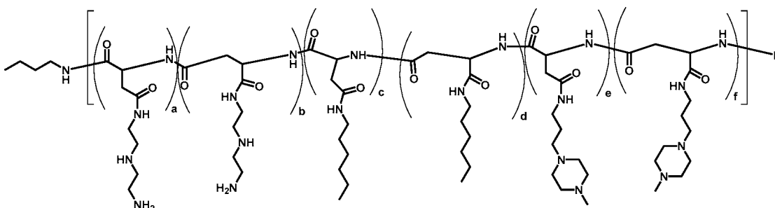
Polymer 57
