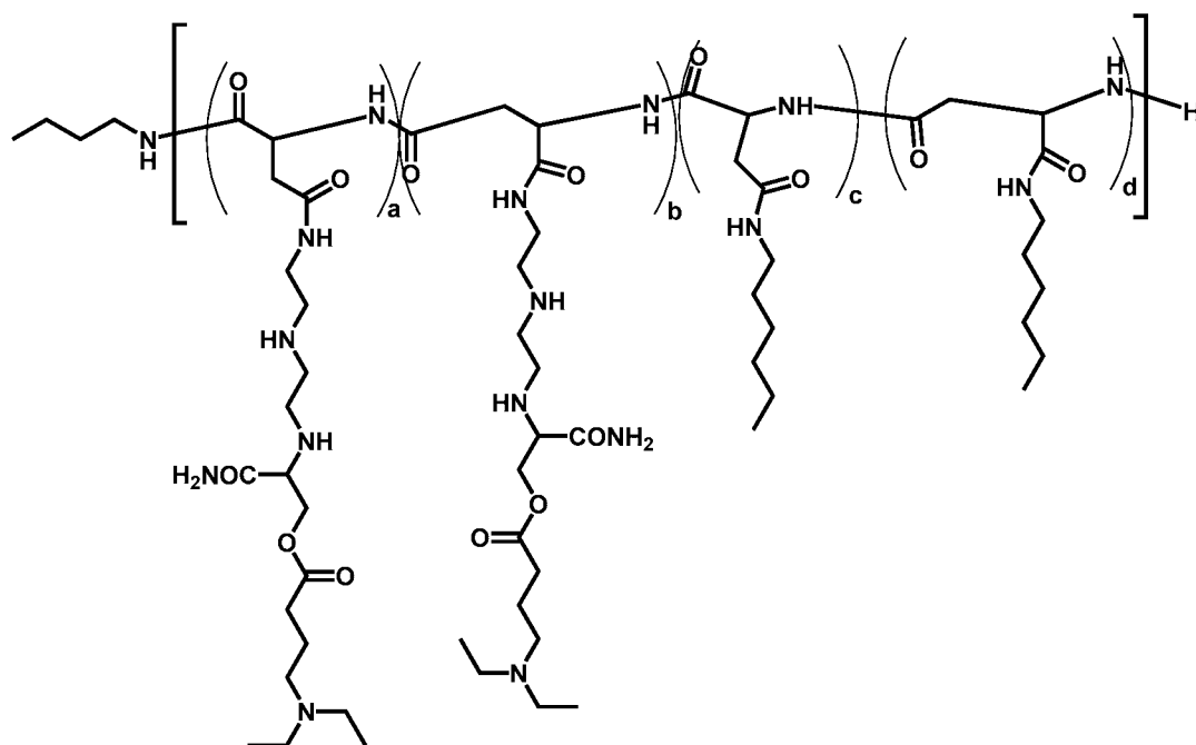
Polymer 61
