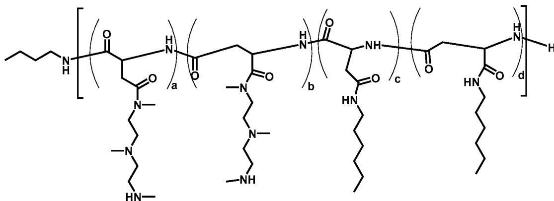
Polymer 40
