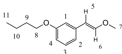
E isomer
