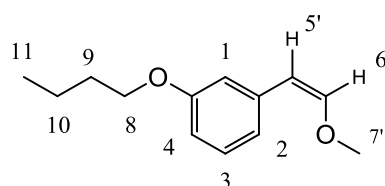
Z isomer
